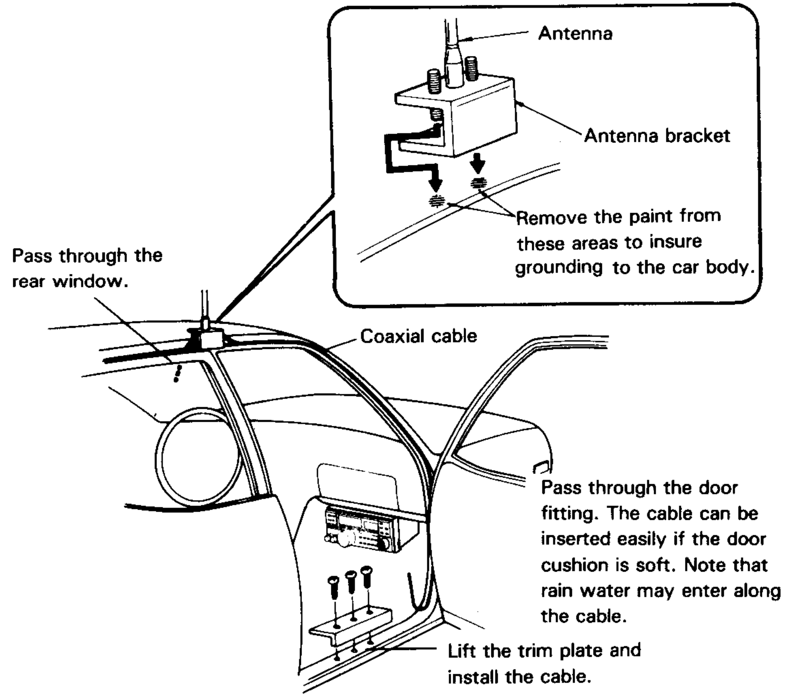
Coax. cable routing
